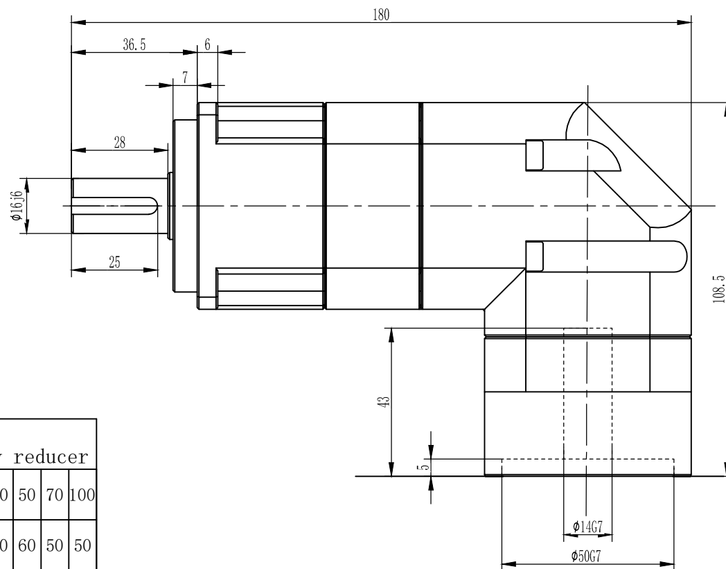
输出端 (Output Terminal)
