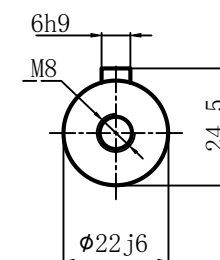
输出端(Output Terminal)
