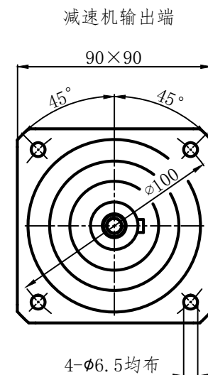
输出端(Output Terminal)
