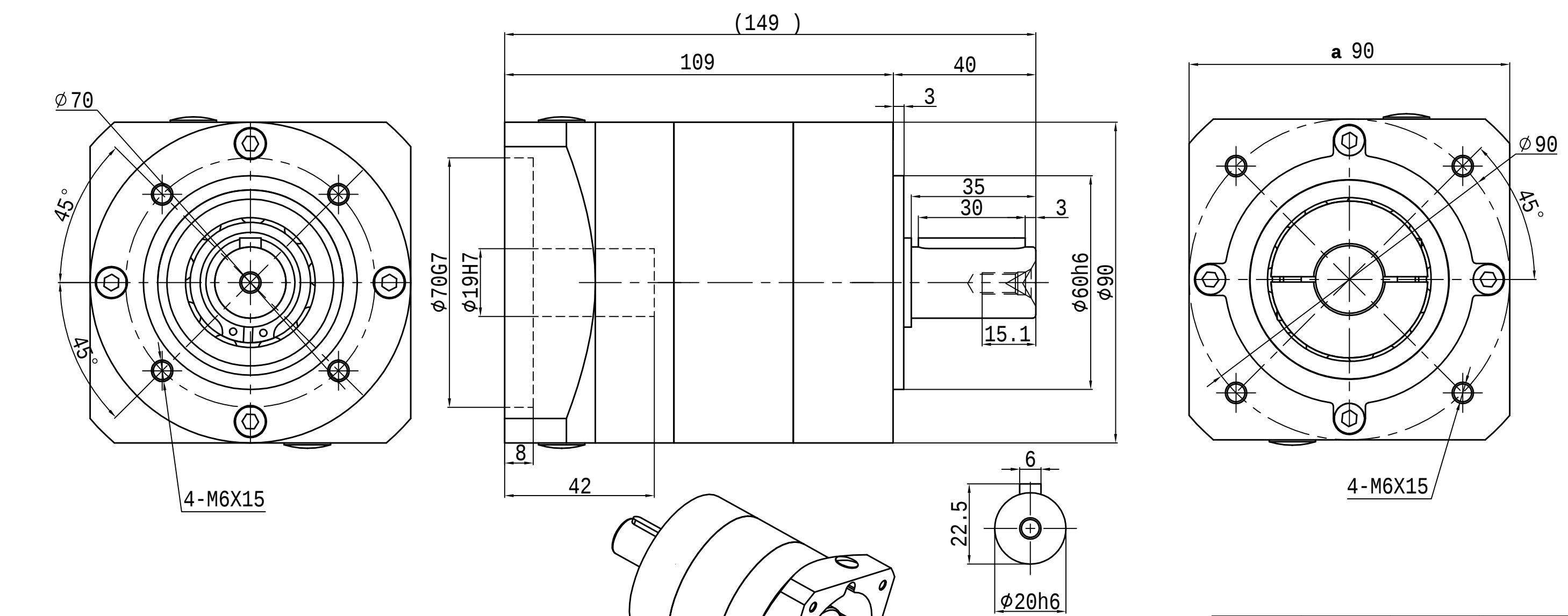
电机尺寸MOTOR DIMENSION: φ19X36/φ70X5/4-φ7-φ90
