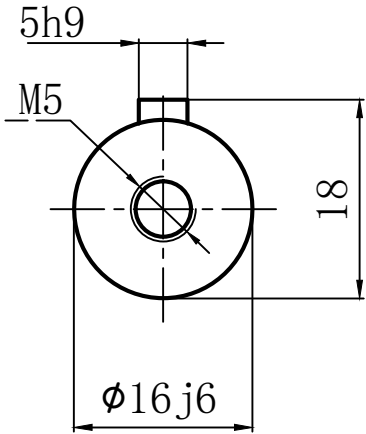
输出端(Output Terminal)
