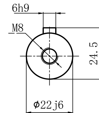
输出端(Output Terminal)
