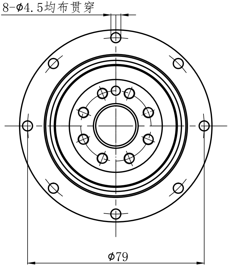
输出端 (Output Terminal)
