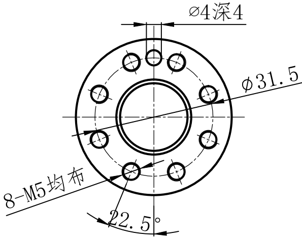
输出端 (Output Terminal)
