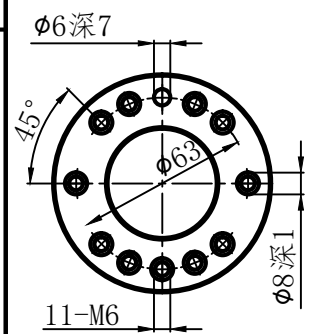
输出端(Output Terminal)
