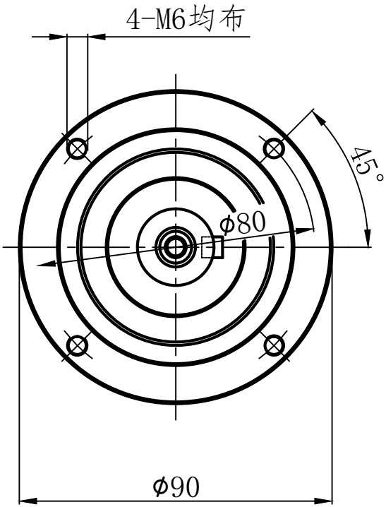
输出端(Output Terminal)
