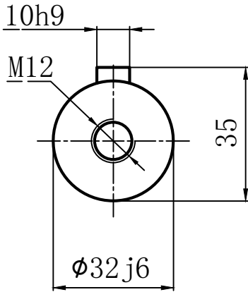
输出端(Output Terminal)
